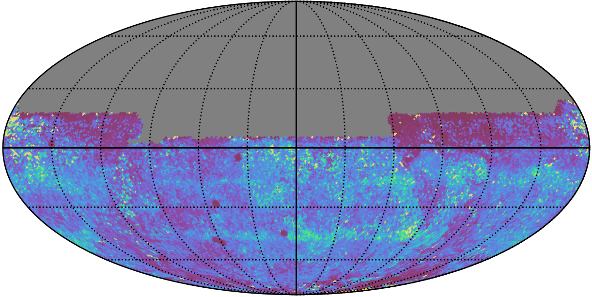
ddf_acor_sf20_lsf30_lsr50_v3.4_10yrs All sky y band: 75th Percentile Intranight Timespan
