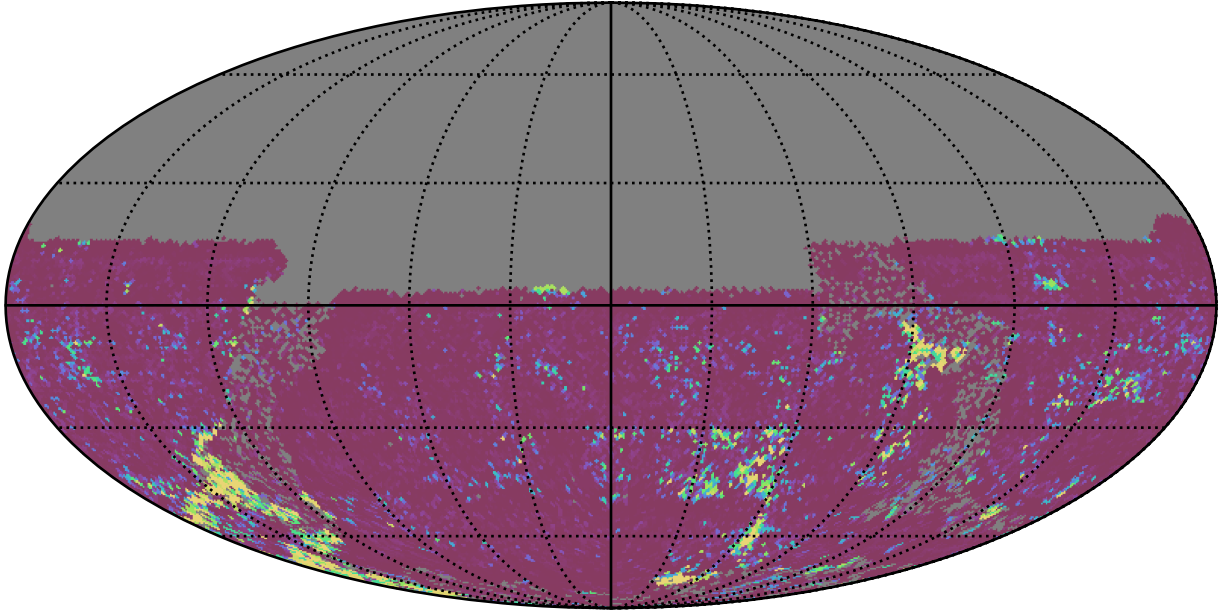
ddf_acor_sf20_lsf30_lsr50_v3.4_10yrs All sky u band: 75th Percentile Intranight Timespan
