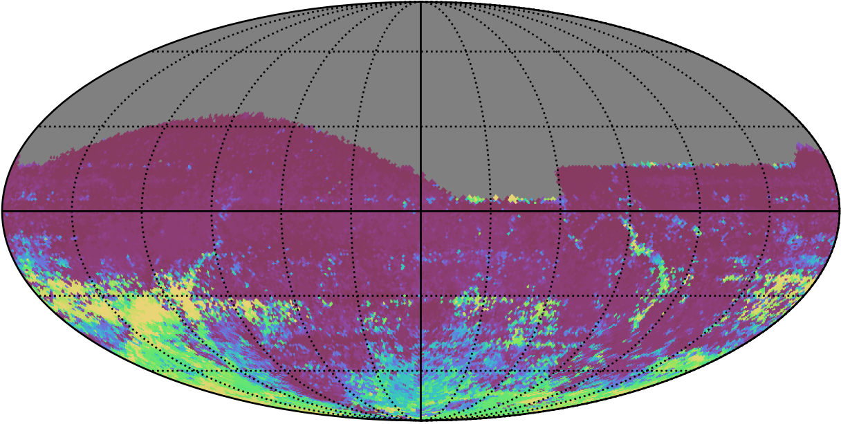
ddf_acor_sf20_lsf30_lsr50_v3.4_10yrs All sky r band: 75th Percentile Intranight Timespan
