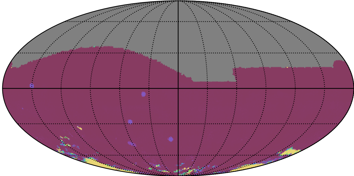
ddf_acor_sf20_lsf30_lsr50_v3.4_10yrs All sky iz bands: 75th Percentile Intranight Timespan
