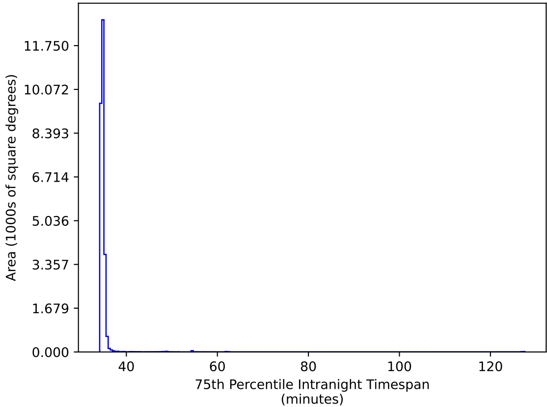
ddf_acor_sf20_lsf30_lsr50_v3.4_10yrs All sky iz bands: 75th Percentile Intranight Timespan
