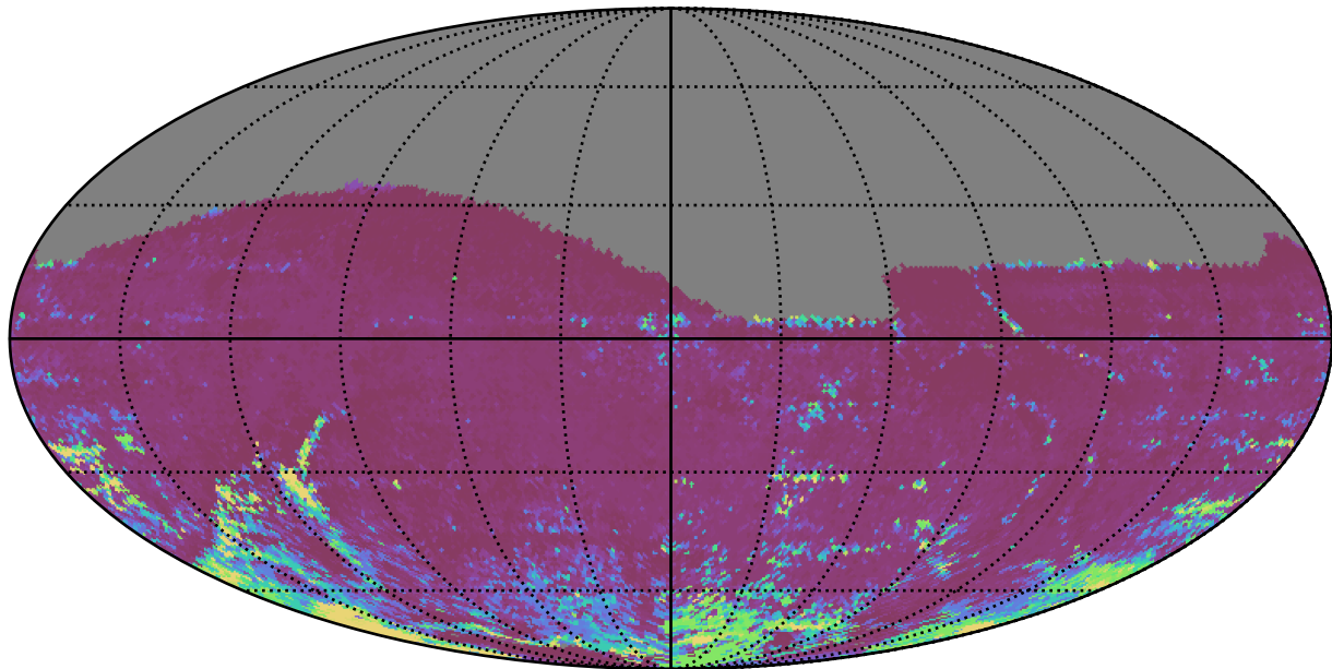
ddf_acor_sf20_lsf30_lsr50_v3.4_10yrs All sky i band: 75th Percentile Intranight Timespan
