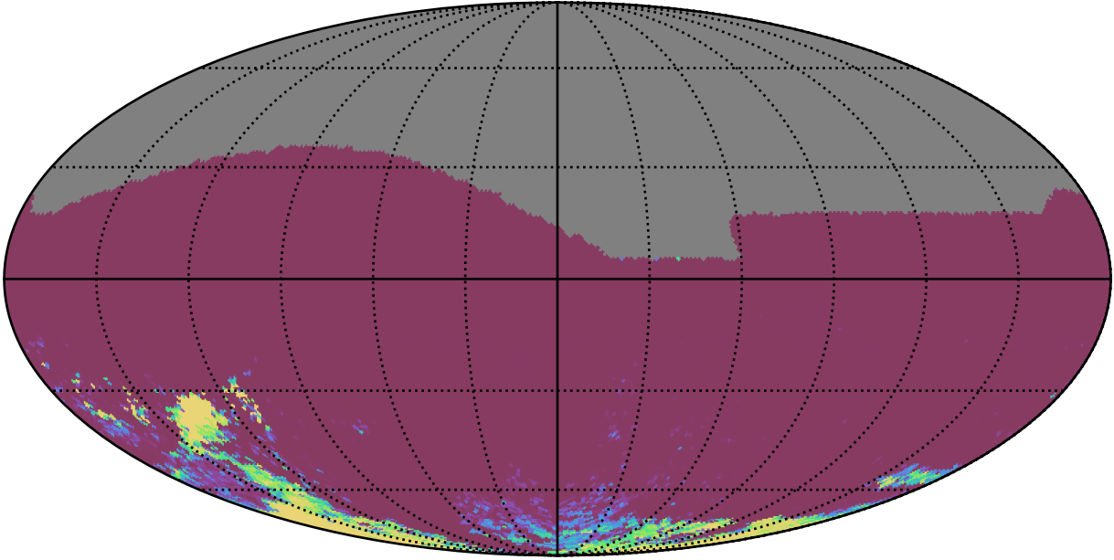
ddf_acor_sf20_lsf30_lsr50_v3.4_10yrs All sky gr bands: 75th Percentile Intranight Timespan
