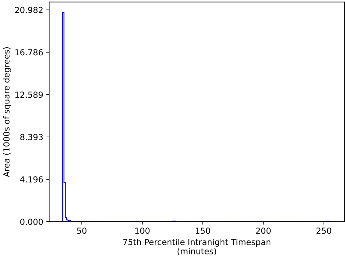
ddf_acor_sf20_lsf30_lsr50_v3.4_10yrs All sky gr bands: 75th Percentile Intranight Timespan
