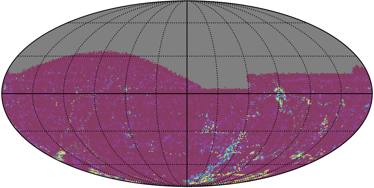
ddf_acor_sf20_lsf30_lsr50_v3.4_10yrs All sky g band: 75th Percentile Intranight Timespan
