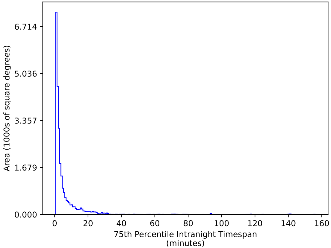
ddf_acor_sf20_lsf30_lsr50_v3.4_10yrs All sky g band: 75th Percentile Intranight Timespan
