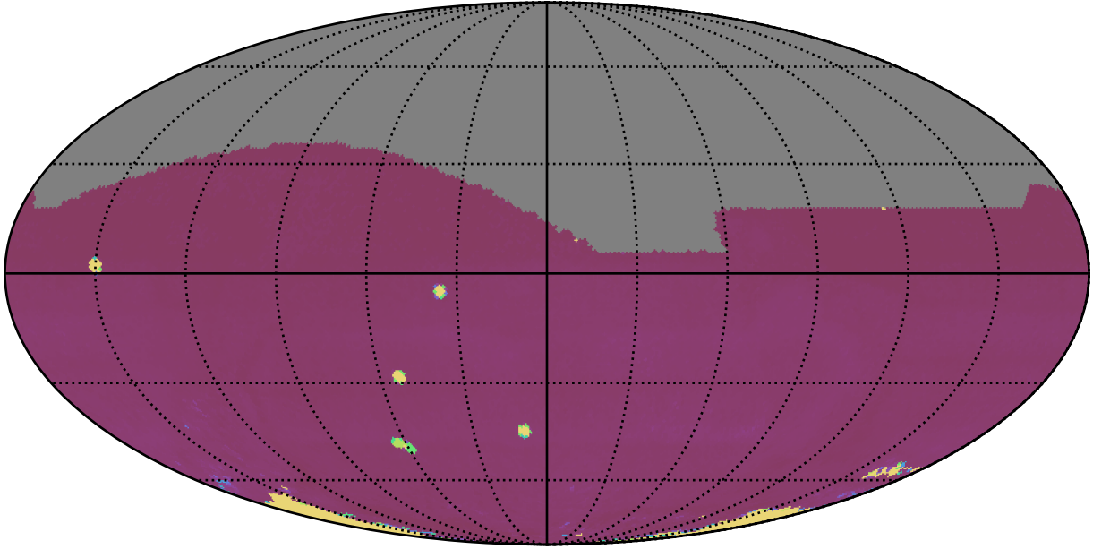
ddf_acor_sf20_lsf30_lsr50_v3.4_10yrs All sky all bands: 75th Percentile Intranight Timespan
