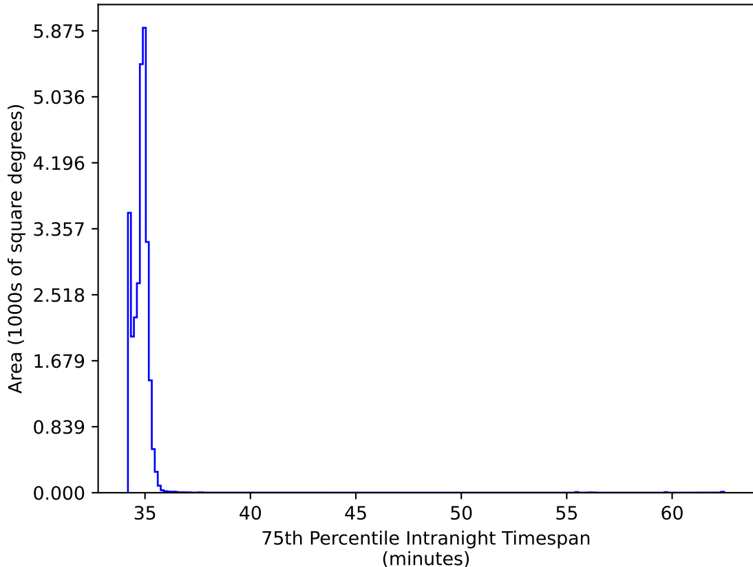
ddf_acor_sf20_lsf30_lsr50_v3.4_10yrs All sky all bands: 75th Percentile Intranight Timespan
