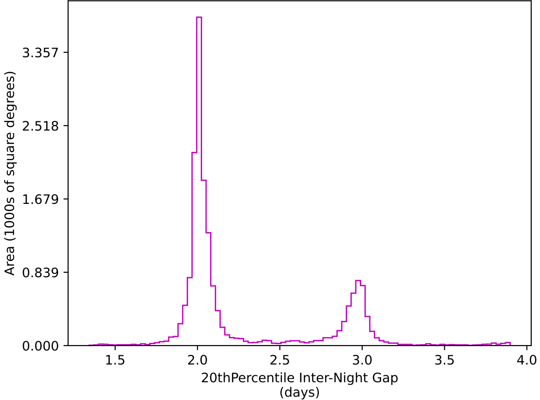
ddf_acor_sf20_lsf30_lsr50_v3.4_10yrs WFD z band: 20thPercentile Inter-Night Gap
