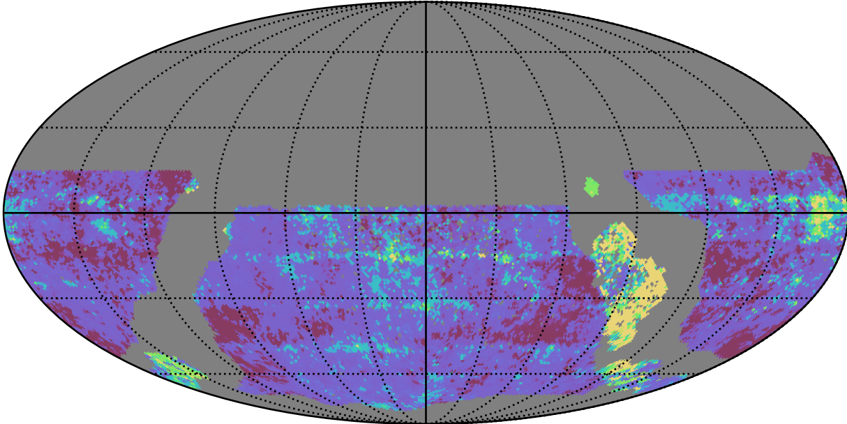
ddf_acor_sf20_lsf30_lsr50_v3.4_10yrs WFD y band: 20thPercentile Inter-Night Gap
