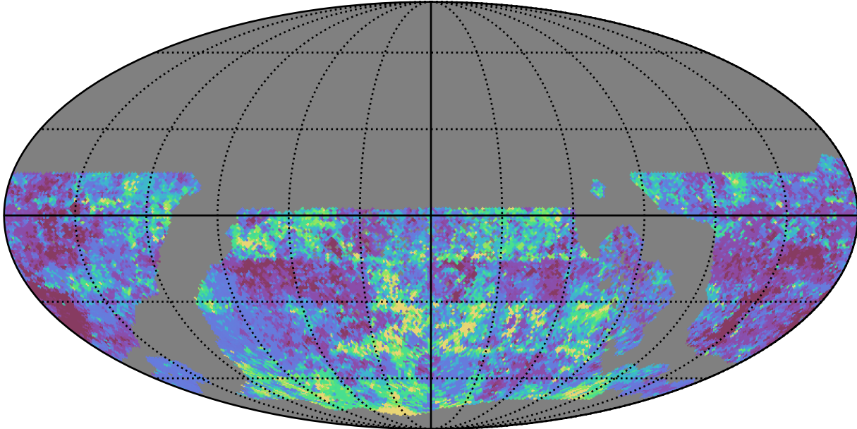
ddf_acor_sf20_lsf30_lsr50_v3.4_10yrs WFD g band: 20thPercentile Inter-Night Gap
