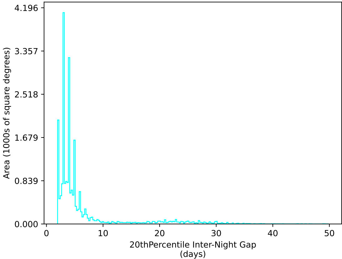
ddf_acor_sf20_lsf30_lsr50_v3.4_10yrs All sky u band: 20thPercentile Inter-Night Gap
