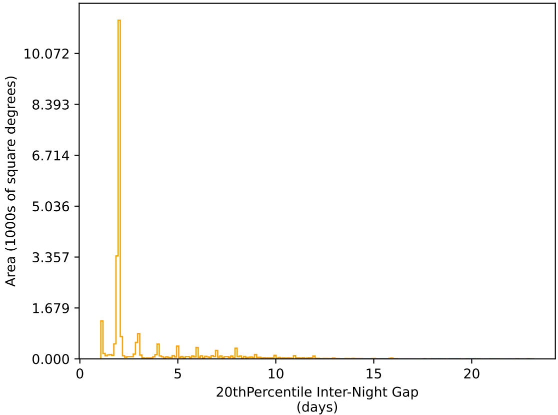
ddf_acor_sf20_lsf30_lsr50_v3.4_10yrs All sky r band: 20thPercentile Inter-Night Gap
