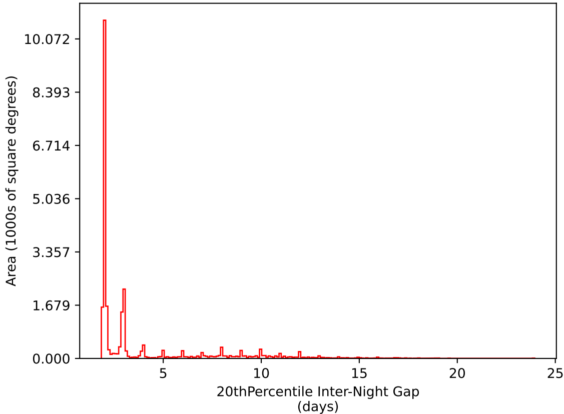
ddf_acor_sf20_lsf30_lsr50_v3.4_10yrs All sky i band: 20thPercentile Inter-Night Gap
