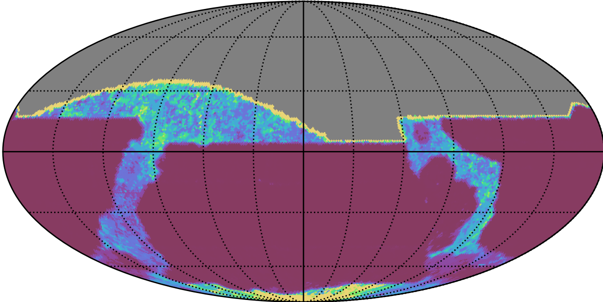
ddf_acor_sf20_lsf30_lsr50_v3.4_10yrs All sky all bands: 20thPercentile Inter-Night Gap
