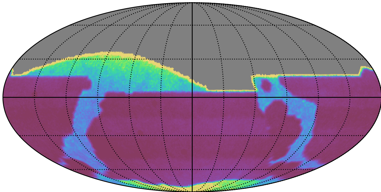
ddf_acor_sf20_lsf30_lsr50_v3.4_10yrs : properMotion
