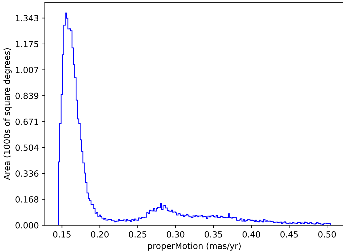
ddf_acor_sf20_lsf30_lsr50_v3.4_10yrs : properMotion
