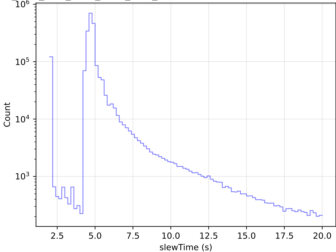
ddf_acor_sf20_Isf30_Isr50_v3.4_10yrs All visits: Zoom Slew Time Histogram
