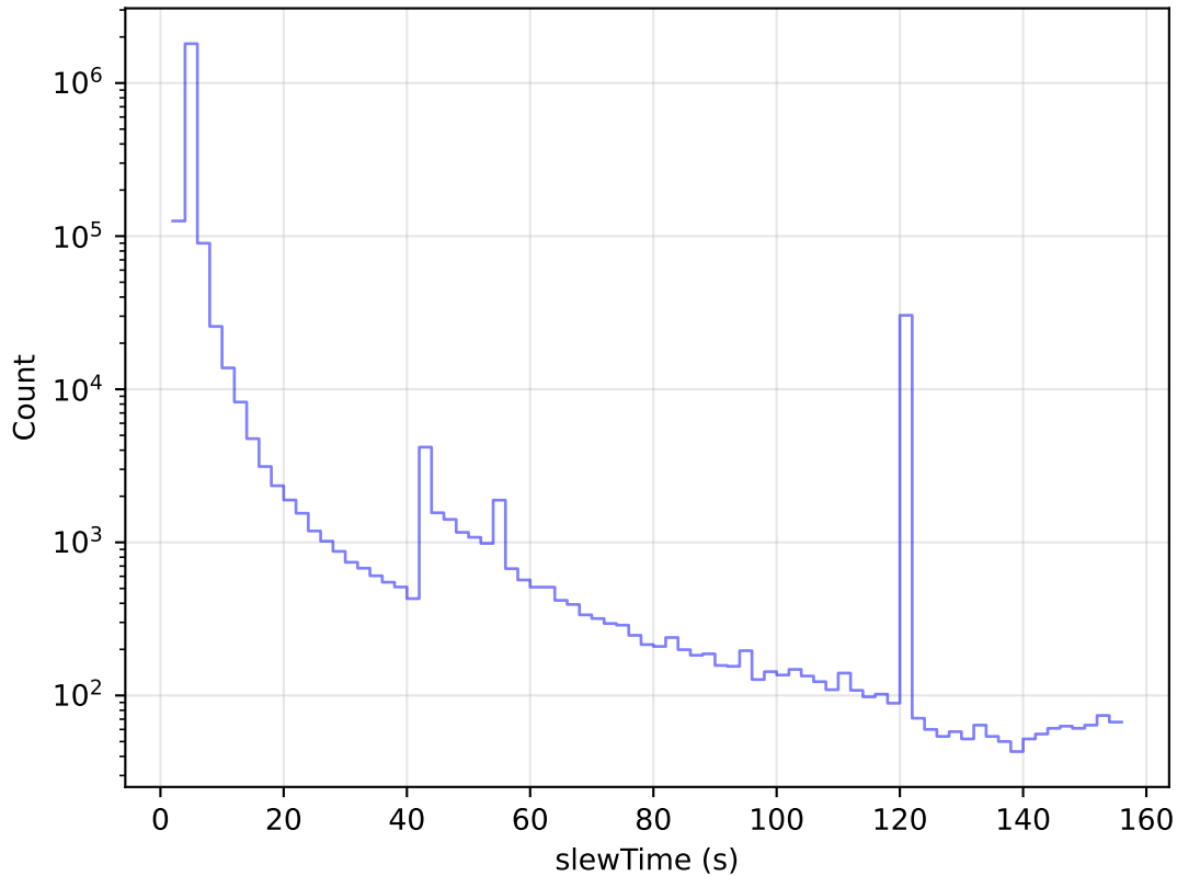
ddf_acor_sf20_lsf30_lsr50_v3.4_10yrs All visits: Slew Time Histogram
