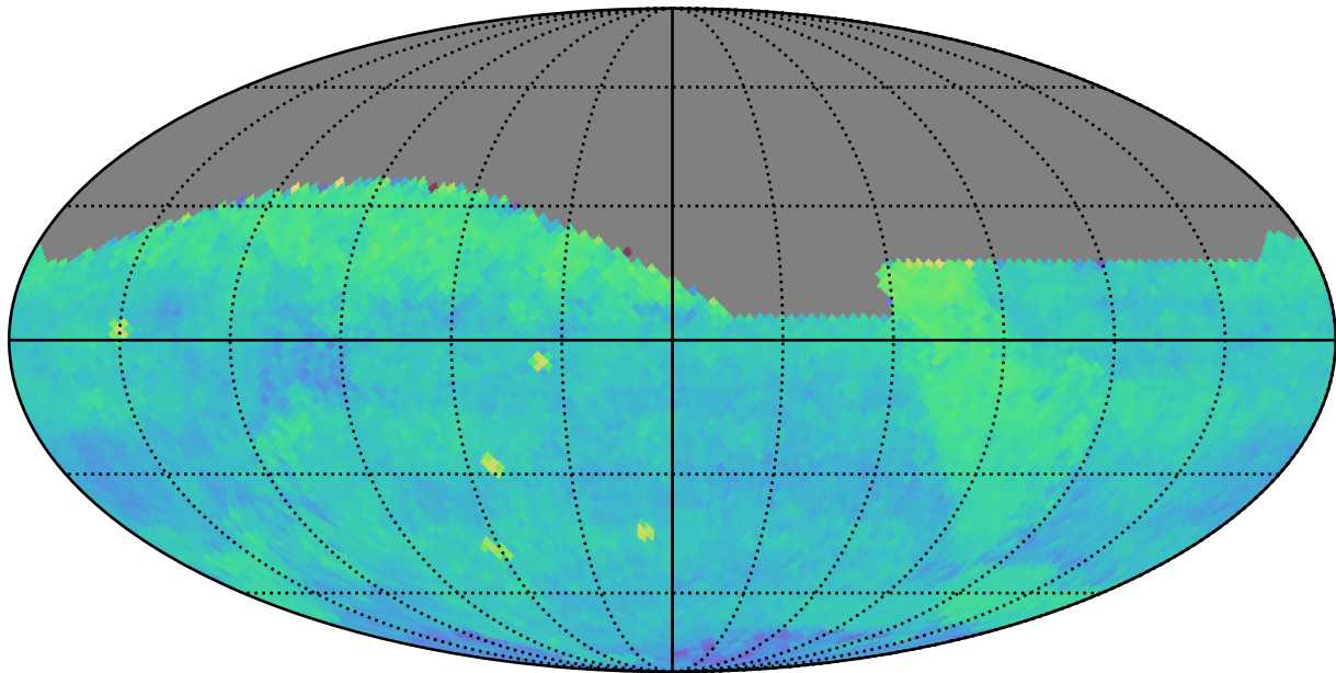
ddf_acor_sf20_lsf30_lsr50_v3.4_10yrs (g or r or i): PairFraction
