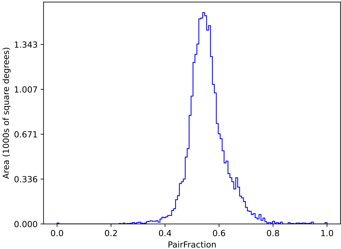
ddf_acor_sf20_lsf30_lsr50_v3.4_10yrs (g or r or i): PairFraction
