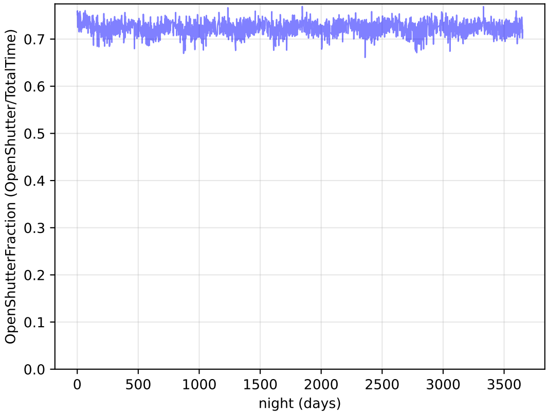
ddf_acor_sf20_lsf30_lsr50_v3.4_10yrs : OpenShutterFraction
