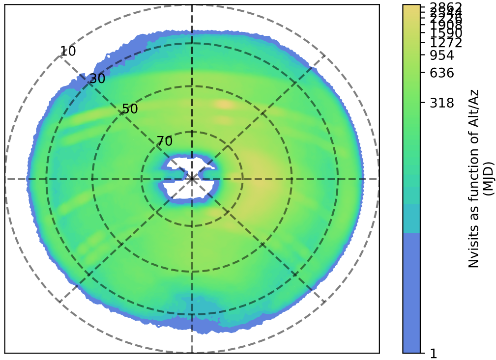
ddf_acor_sf20_lsf30_lsr50_v3.4_10yrs z: Nvisits as function of Alt/Az
