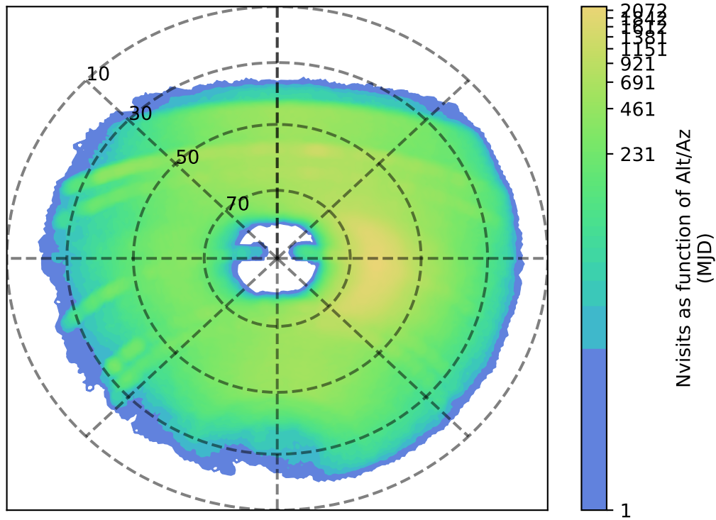
ddf_acor_sf20_lsf30_lsr50_v3.4_10yrs y: Nvisits as function of Alt/Az
