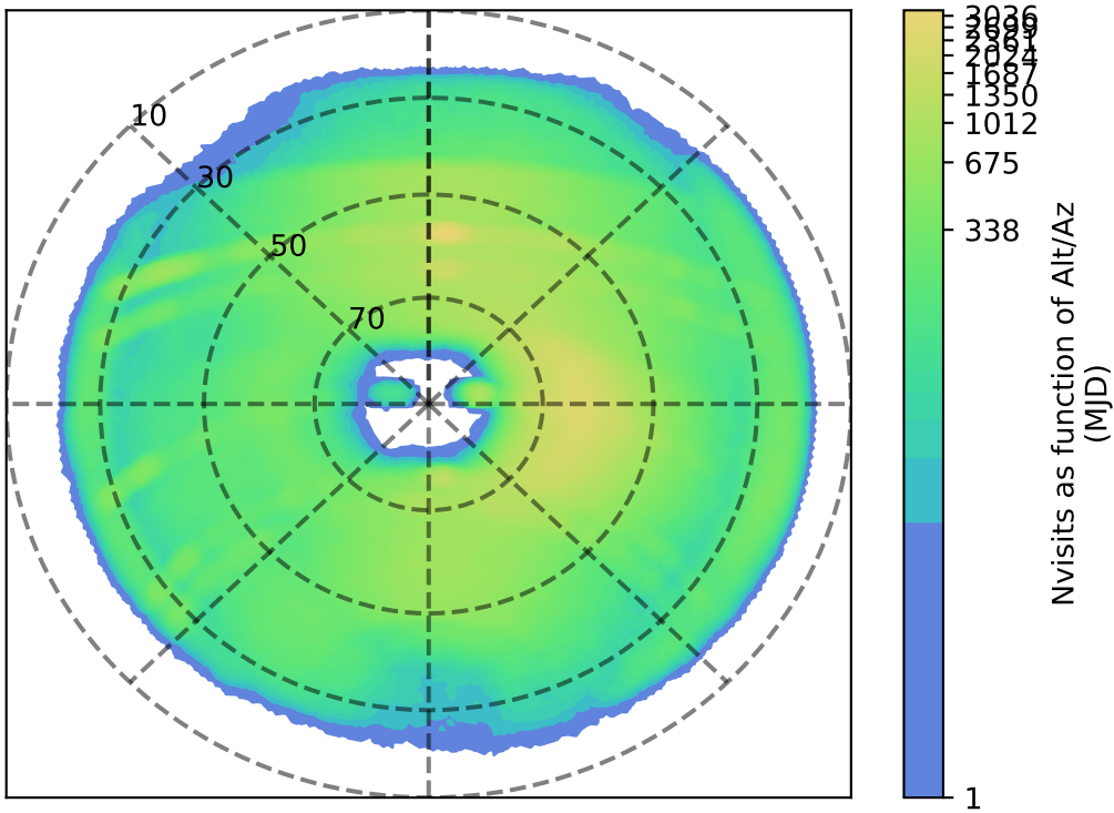
ddf_acor_sf20_ls30_lsr50_v3.4_10yrs i: Nvisits as function of Alt/Az
