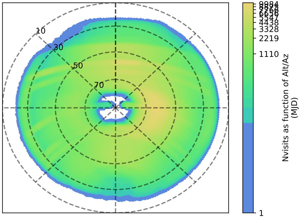
ddf_acor_sf20_lsf30_lsr50_v3.4_10yrs : Nvisits as function of Alt/Az
