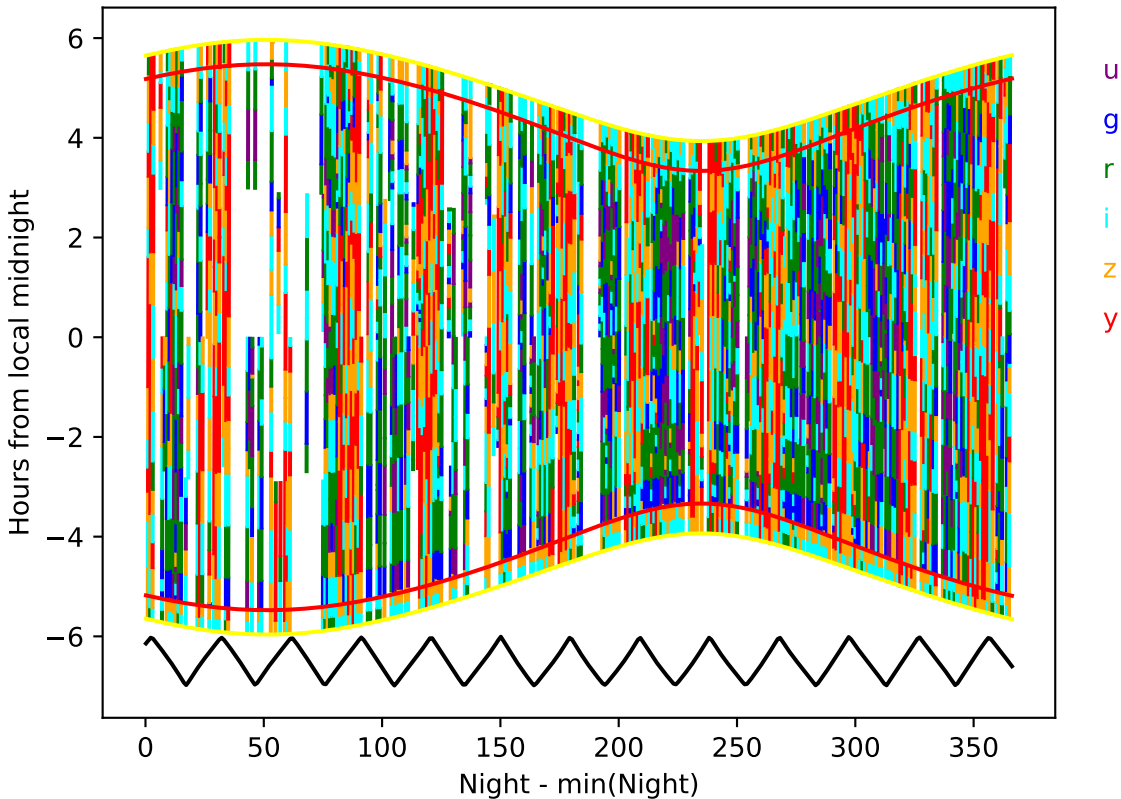
ddf_acor_sf20_lsf30_lsr50_v3.4_10yrs year 9-10: Hourglass
