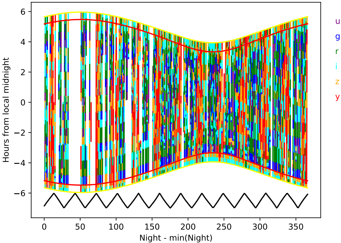
ddf_acor_sf20_lsf30_lsr50_v3.4_10yrs year 8-9: Hourglass
