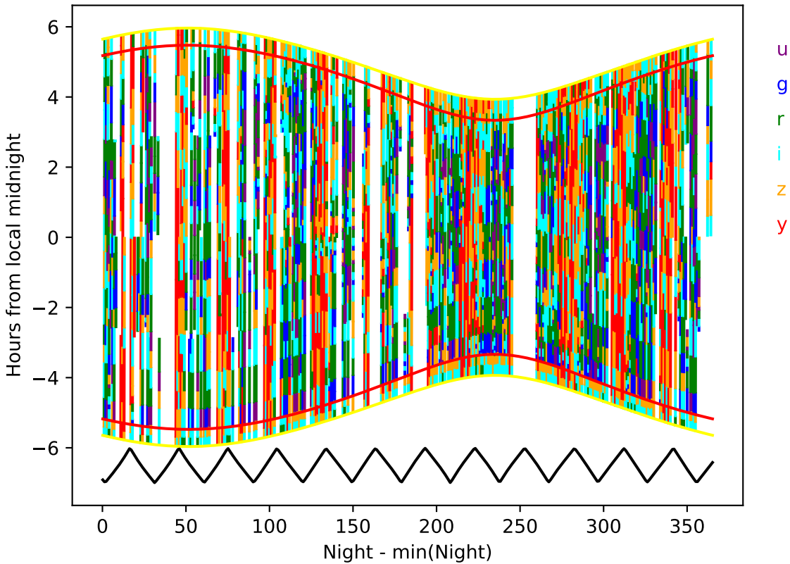
ddf_acor_sf20_lsf30_lsr50_v3.4_10yrs year 5-6: Hourglass
