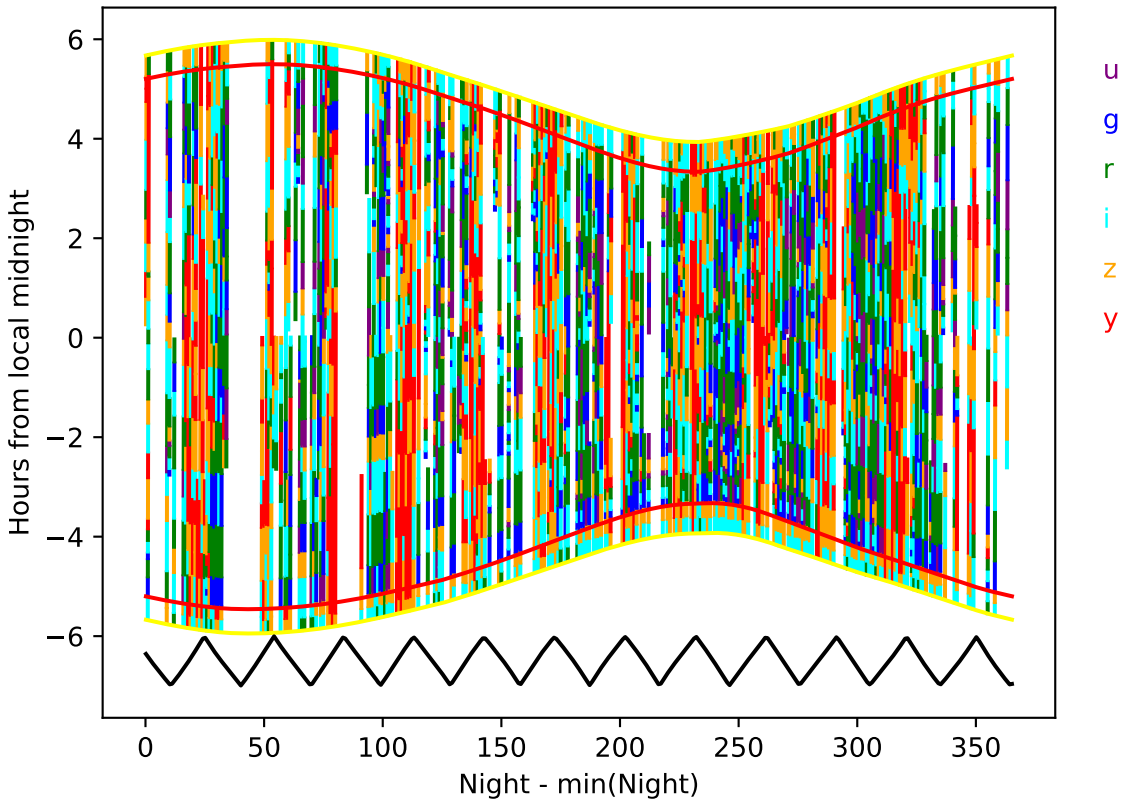
ddf_acor_sf20_lsf30_lsr50_v3.4_10yrs year 4-5: Hourglass
