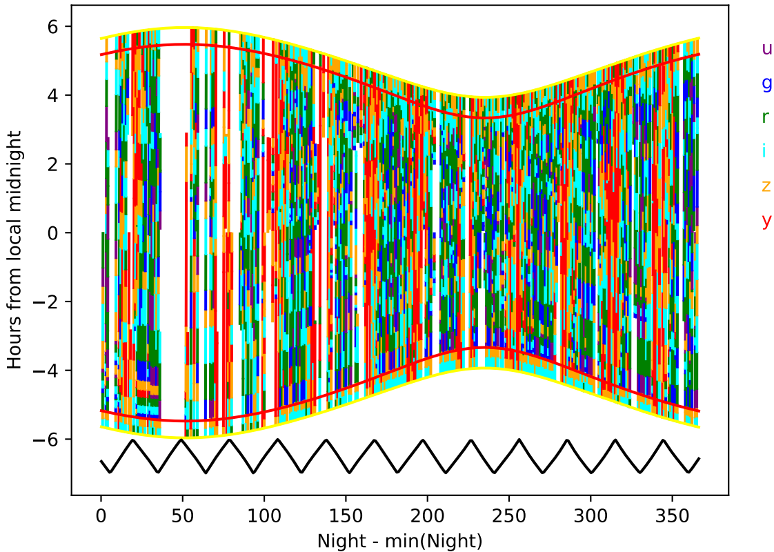
ddf_acor_sf20_lsf30_lsr50_v3.4_10yrs year 2-3: Hourglass
