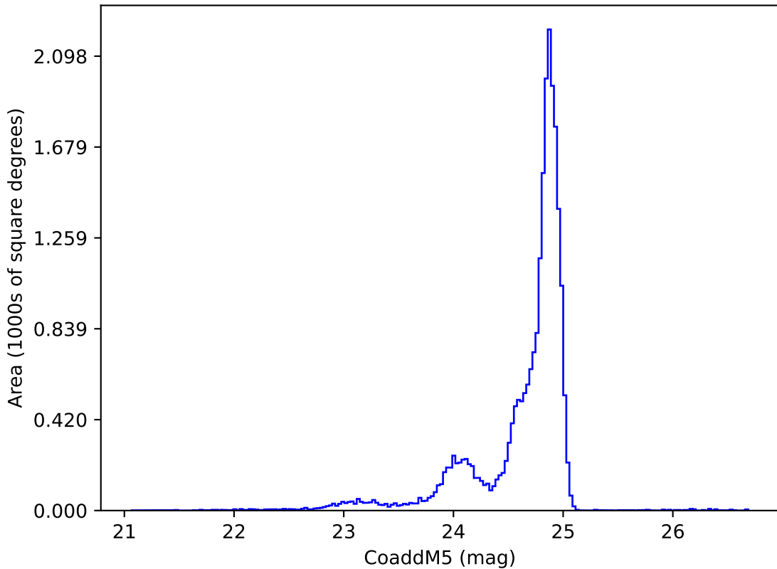
ddf_acor_sf20_lsf30_lsr50_v3.4_10yrs y: CoaddM5
