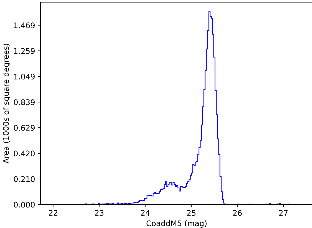
ddf_acor_sf20_lsf30_lsr50_v3.4_10yrs u: CoaddM5
