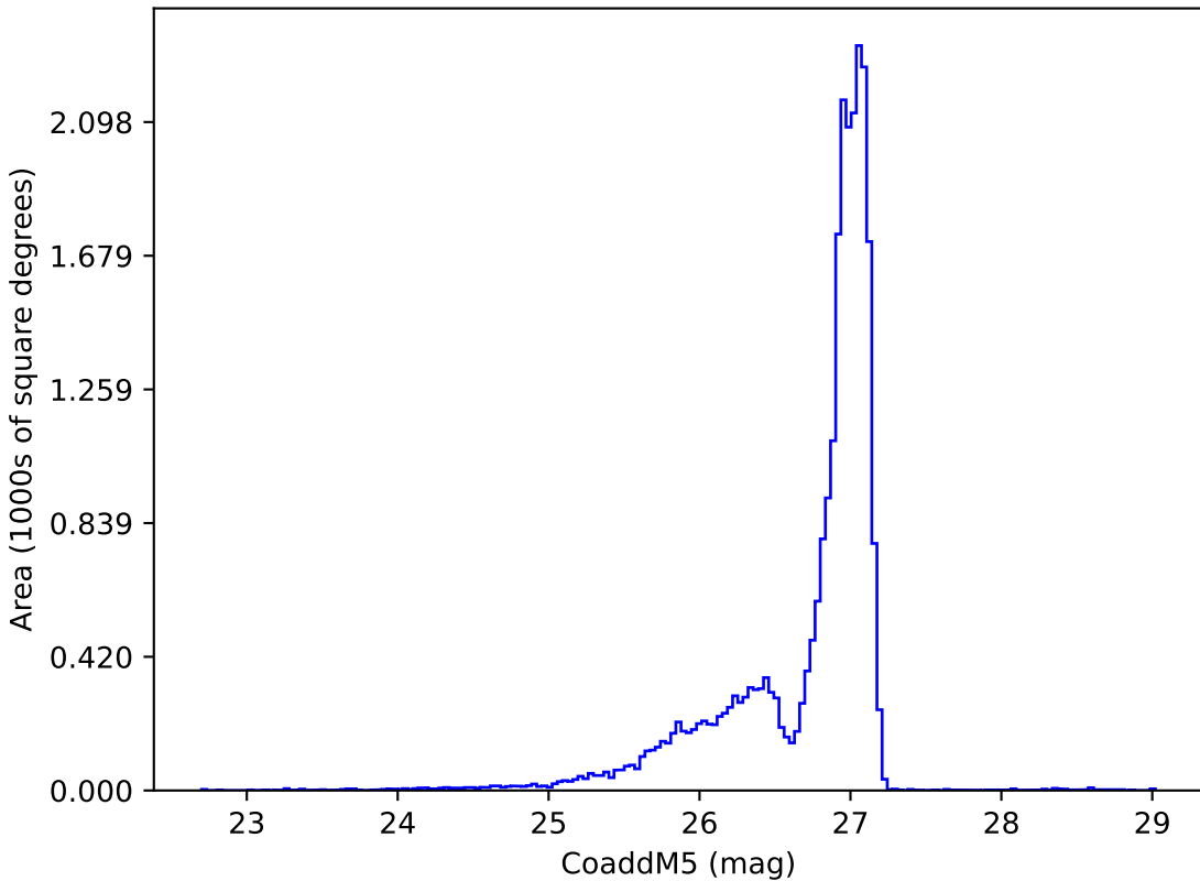
ddf_acor_sf20_lsf30_lsr50_v3.4_10yrs r: CoaddM5
