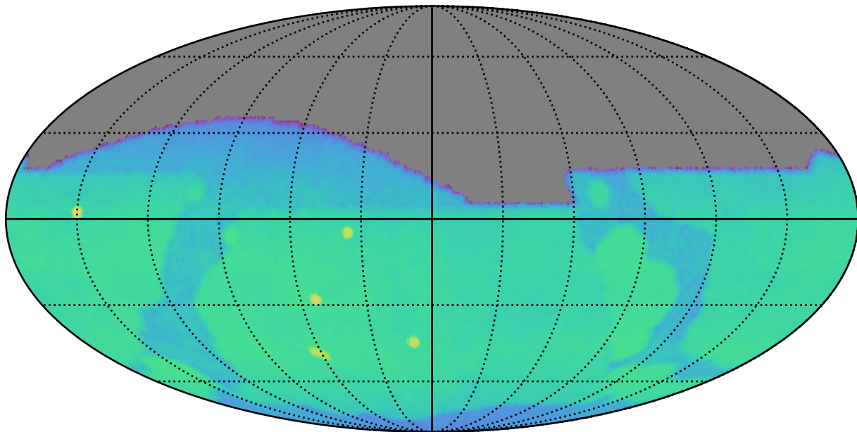
ddf_acor_sf20_lsf30_lsr50_v3.4_10yrs g: CoaddM5
