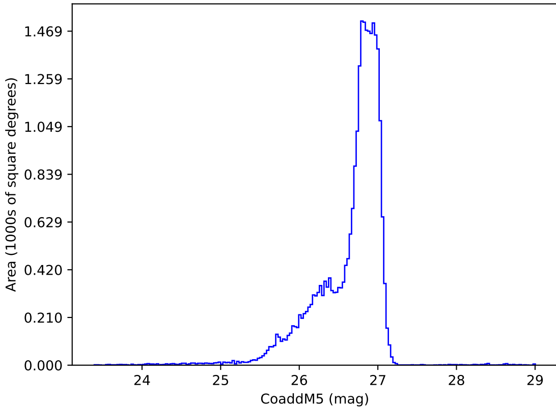
ddf_acor_sf20_ls30_lsr50_v3.4_10yrs g: CoaddM5
