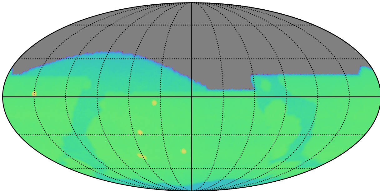
ddf_acor_sf20_lsf30_lsr50_v3.4_10yrs : CoaddM5
