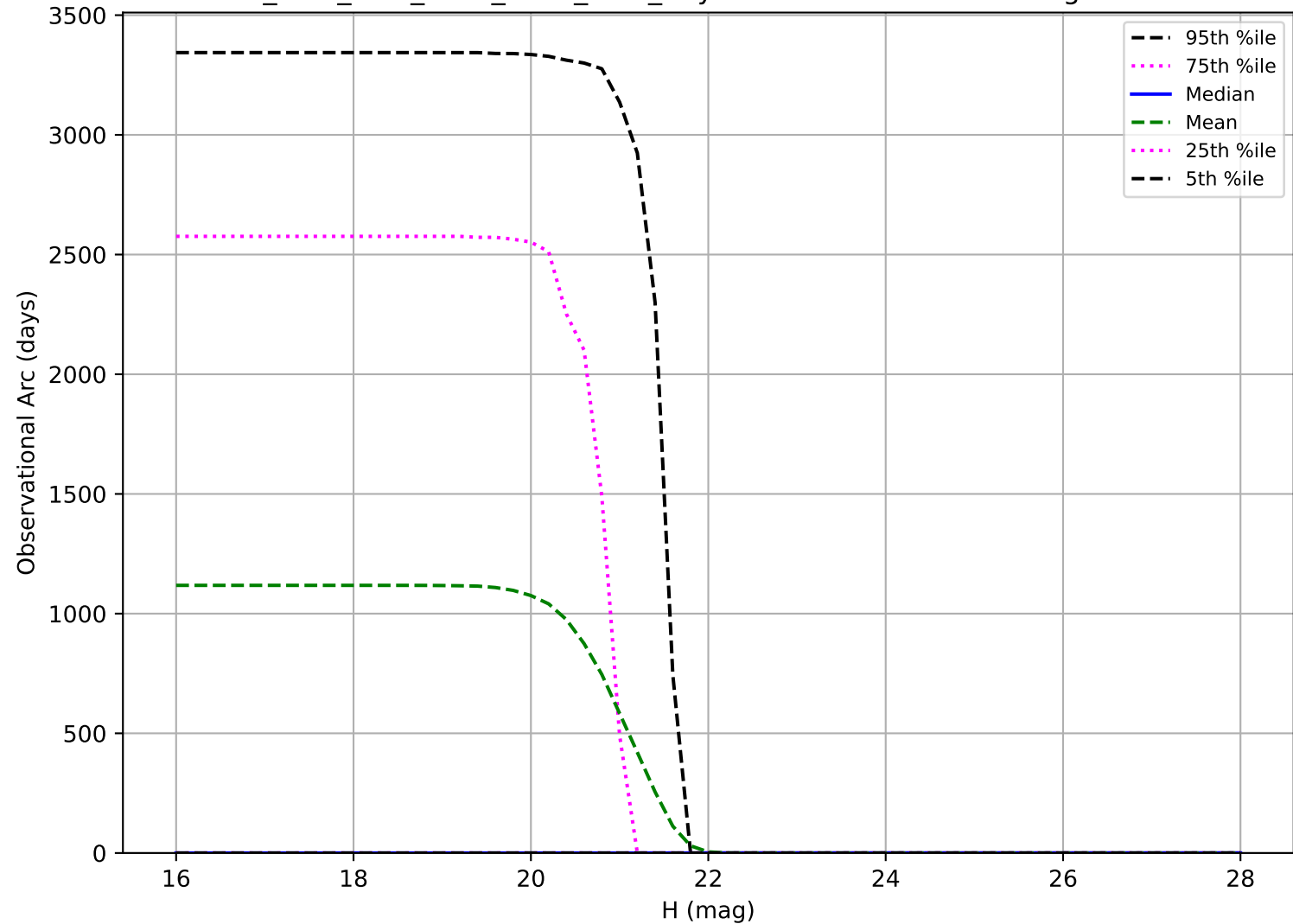
ddf_acor_sf20_lsf30_lsr20_v3.4_10yrs: Observational Arc Length Vatira
