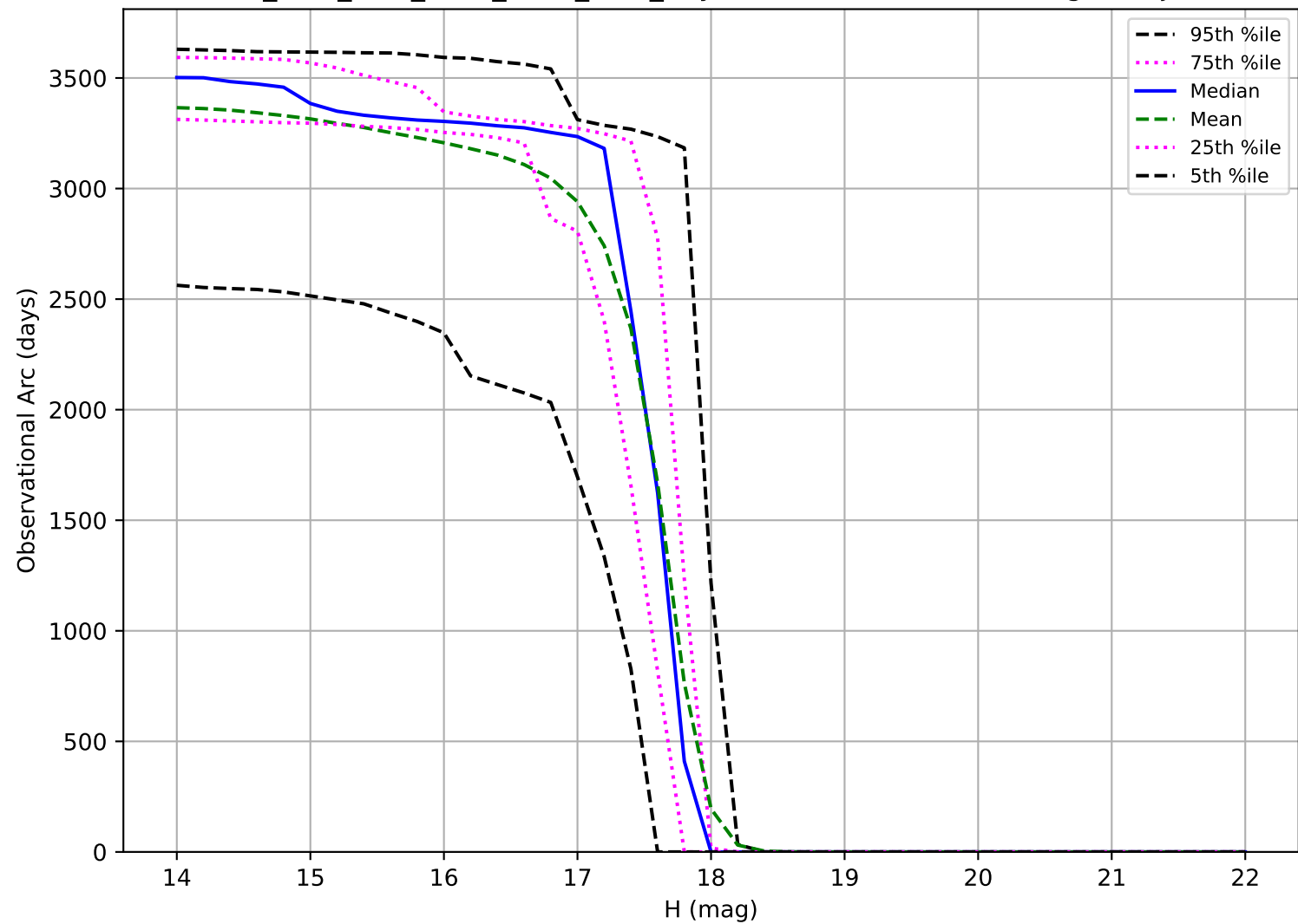
ddf_acor_sf20_lsf30_lsr20_v3.4_10yrs: Observational Arc Length Trojan
