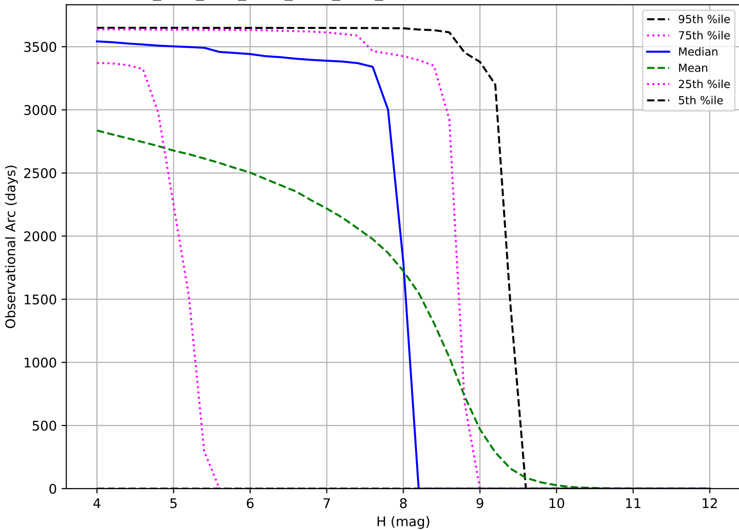
ddf_acor_sf20_Isf30_Isr20_v3.4_10yrs: Observational Arc Length TNO
