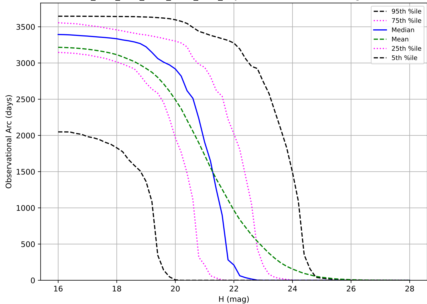
ddf_acor_sf20_lsf30_lsr20_v3.4_10yrs: Observational Arc Length PHA
