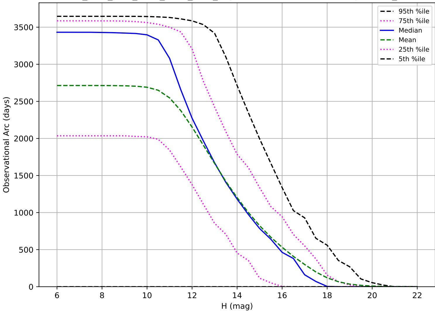
ddf_acor_sf20_lsf30_lsr20_v3.4_10yrs: Observational Arc Length OCC_r5
