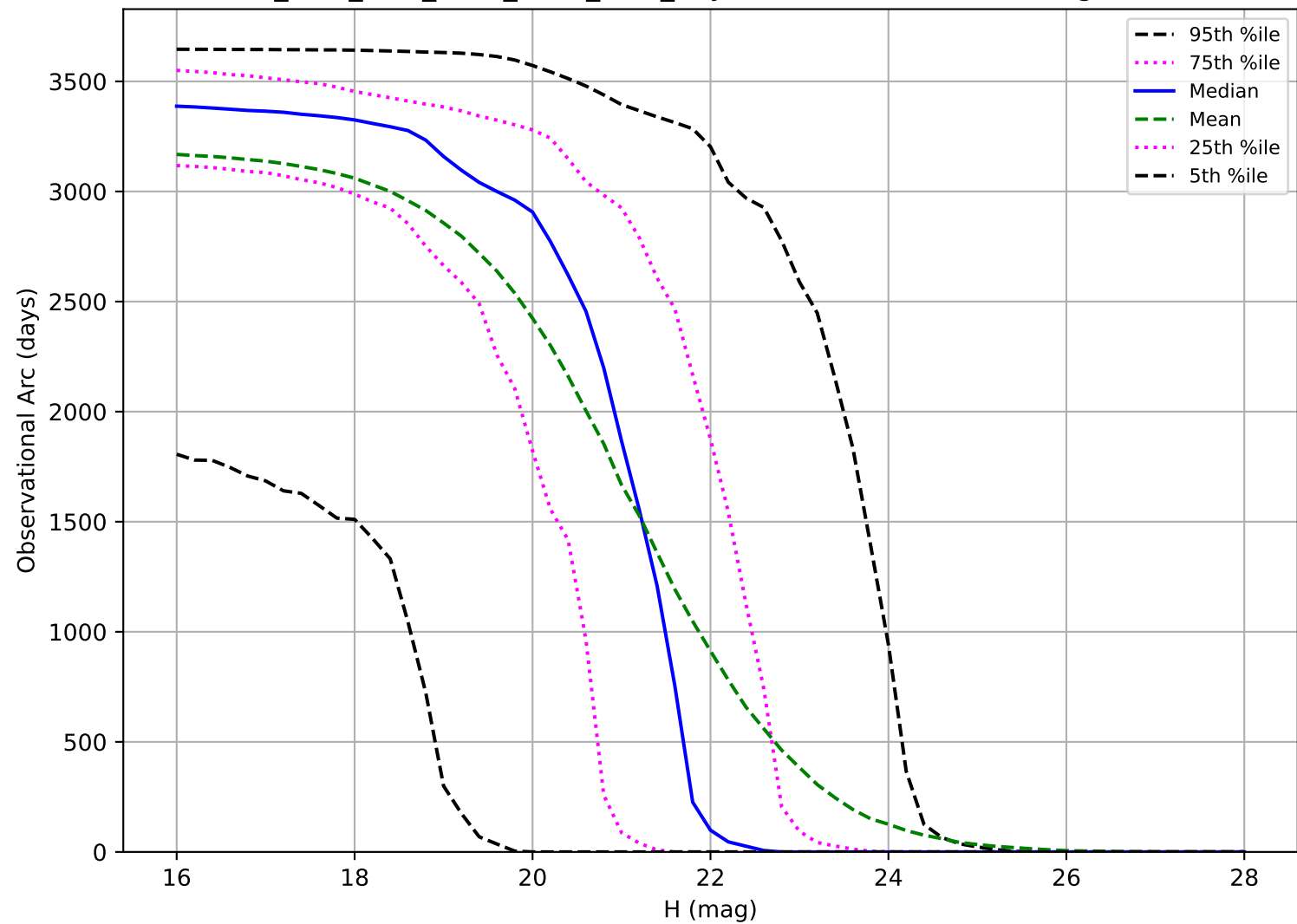
ddf_acor_sf20_lsf30_lsr20_v3.4_10yrs: Observational Arc Length NEO
