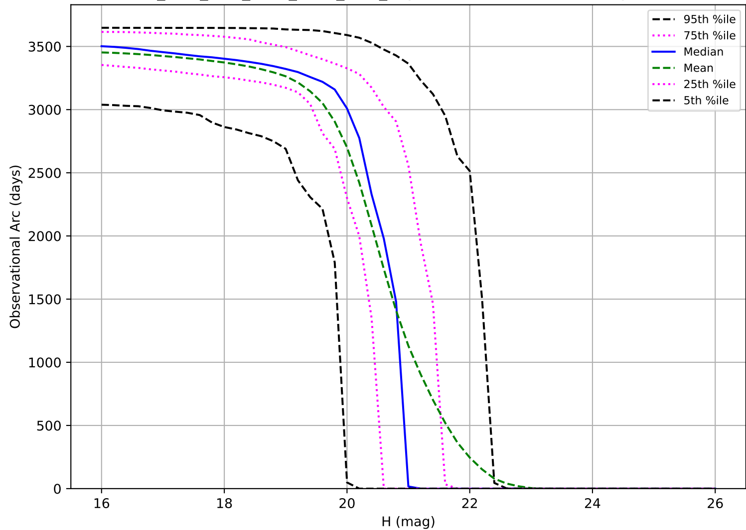
ddf_acor_sf20_lsf30_lsr20_v3.4_10yrs: Observational Arc Length MBA
