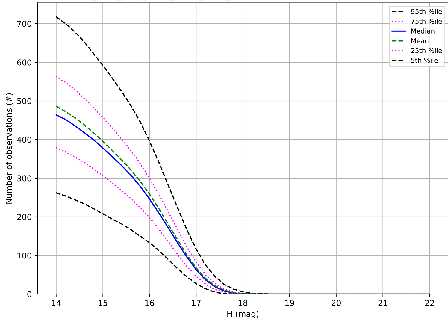
ddf_acor_sf20_lsf30_lsr20_v3.4_10yrs: Number of observations Trojan
