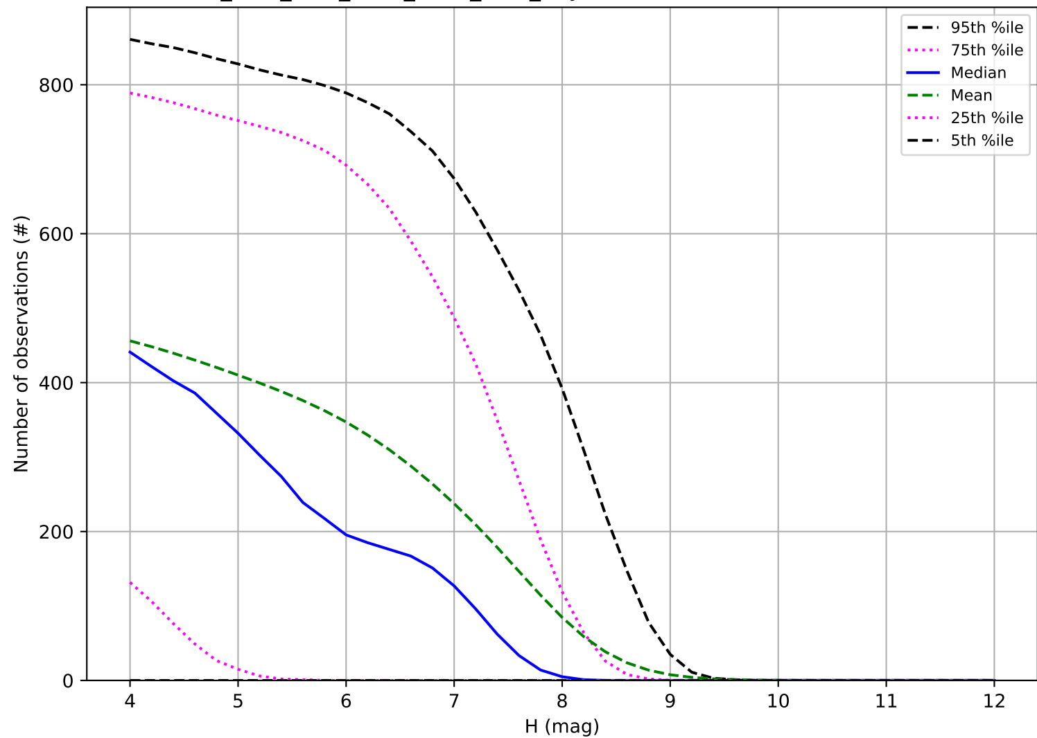
ddf_acor_sf20_lsf30_lsr20_v3.4_10yrs: Number of observations TNO
